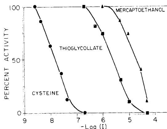
FIG. 2.—Inhibition of zinc carboxypeptidase by mercaptans. 1 \times 10^{-6} M [(\text{CPD})\text{Zn}] was incubated with increasing concentrations of mercaptoethanol, \Delta , thioglycolic acid, \blacksquare , and L-cysteine, \bullet , in 1 M NaCl-0.1 M Tris, pH 7.0, for 72 hours at 0°, under \text{N}_2 . Peptidase activities were measured as in Figure 1 after incubation with mercaptoethanol and thioglycolic acid. Esterase activities were measured after incubation with L-cysteine using 2 \times 10^{-8} M enzyme and 0.01 M hippuryl-DL-phenyl lactic acid in 1 M NaCl-0.005 M Tris, pH 7.5, 25°. The concentration of dissociated inhibitor 3 is plotted as a function of the partial activity expressed as per cent of the uninhibited enzyme acting as a control.
